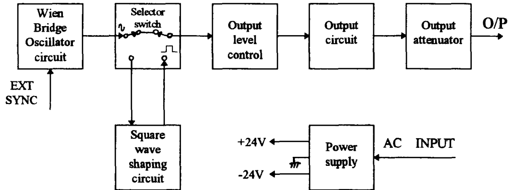
Fig. 1 Block Diagram
